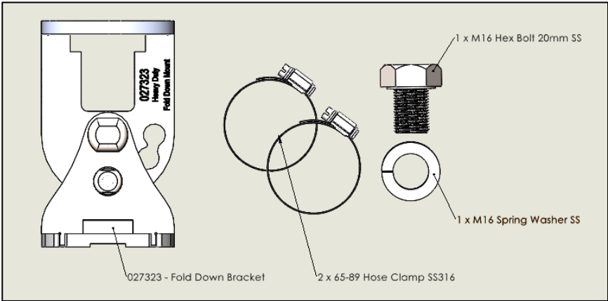
Figure 1. Supplied Components
