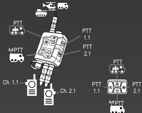
INTERCOM + TWO RADIOS, ONE CHANNEL
