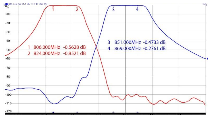
Duplexer Configuration
