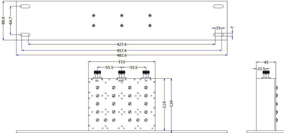
Duplexer Configuration
