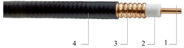
1: Inner Conductor 2: Insulation 3: Outer conductor 4: Jacket
