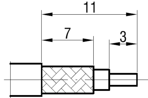
Cable Stripping Dimensions (mm)
