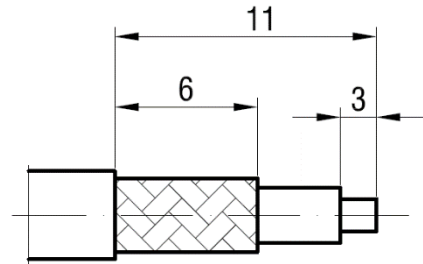
Cable Stripping Dimensions (mm)
