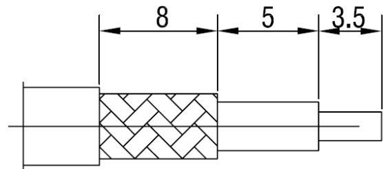
Cable Crimping Dimensions
