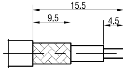
Cable Stripping Dimensions(mm)
