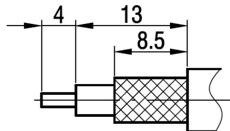
Cable Stripping Dimensions (mm)
