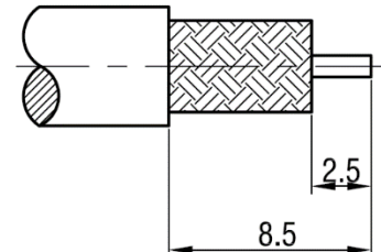
Cable Stripping Dimensions(mm)
