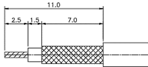
Cable Stripping Dimensions (mm)
