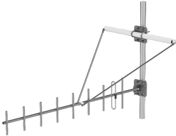
Vertical Polarisation Configuration (Yagi Antenna not included)
