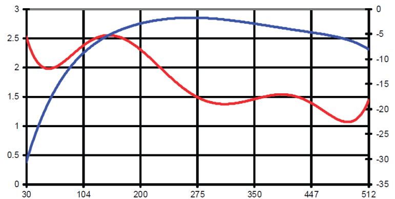
VSWR & GAIN 30-512 MHz Gain (dBi) 30-512 MHz VSWR
