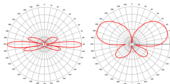
E Plane 896 MHz
