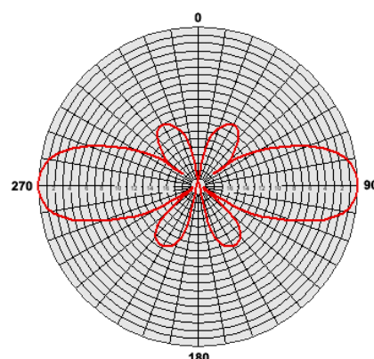
Typical Radiation Pattern
