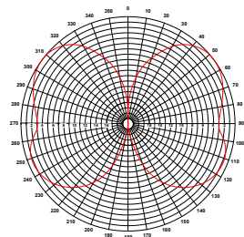
E Plane 690MHz
