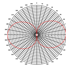
E Plane 1710MHz
